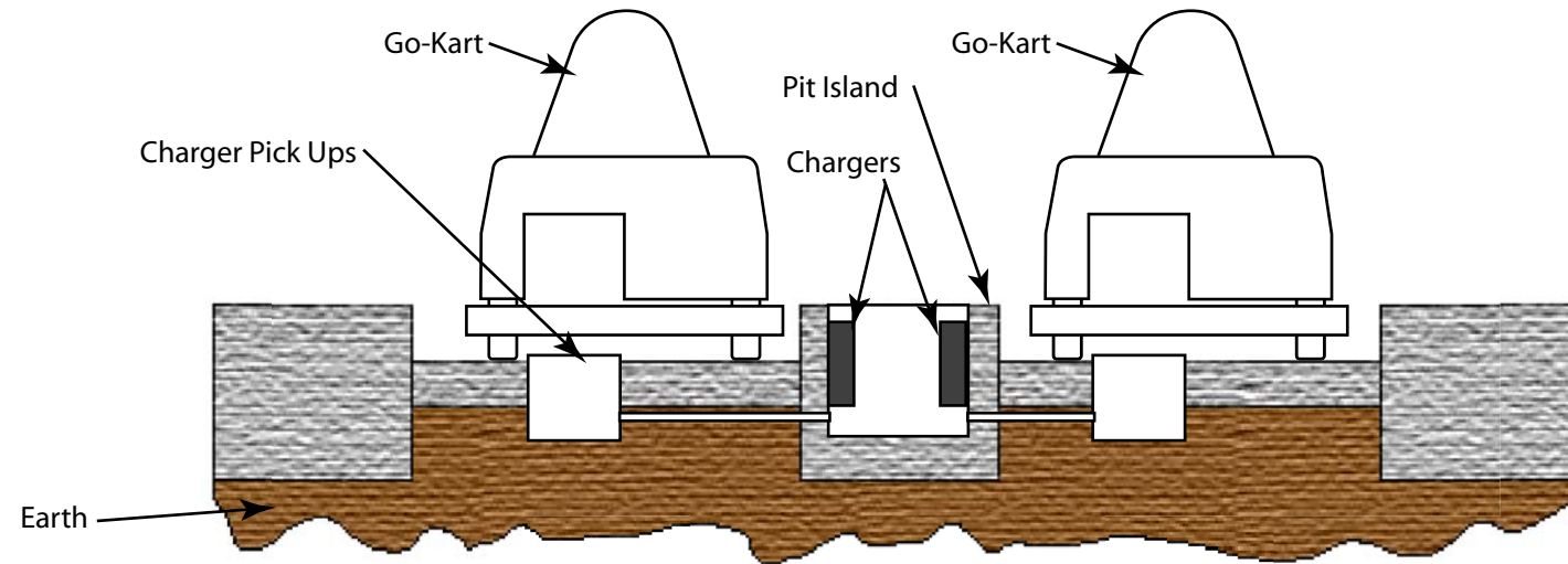
Section View
